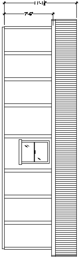
3 REAR ELEVATION SCALE: 1/4" = 1'-0"
