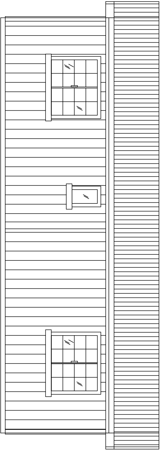
REAR ELEVATION
